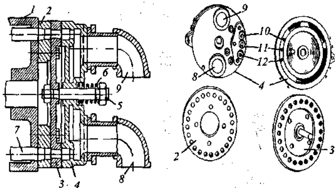
57- rasm. Vakuum-filtr taqsimlovchi kallagining tuzilish sxemasi:
