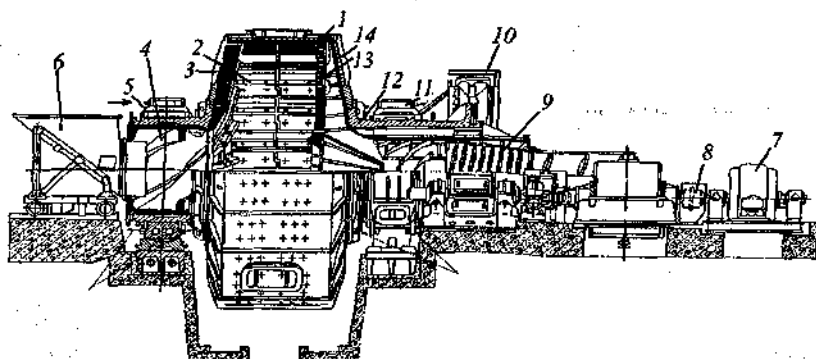
22-rasm. O'z-o'zini yanchuvchi tegirmon MMC 7000x2300.
