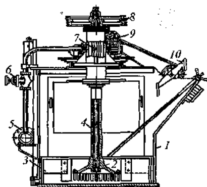
40- rasm. Pnevnomexanik flotatsion mashina:
