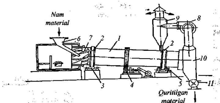
59- rasm. Barabanli quritkich:
