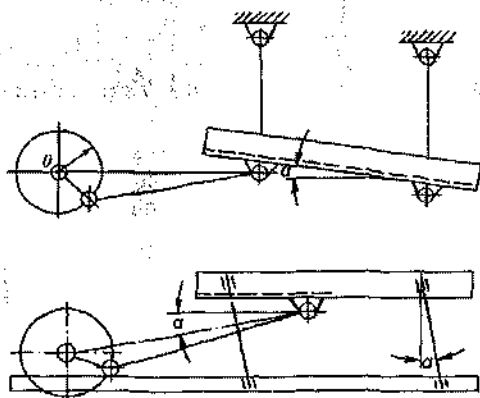
7-rasm. Yassi tebranuvchi elaklar.
