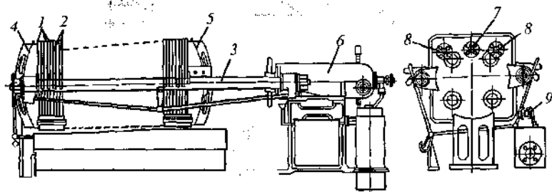
55- rasm. Filtr-press:
