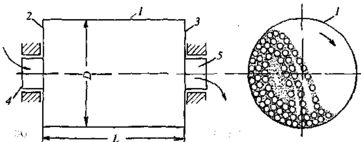
14-rasm. Barabanli tegirmon:
