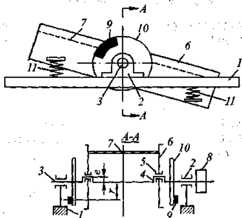
8-rasm. Yarim vibratsion elaklar:
